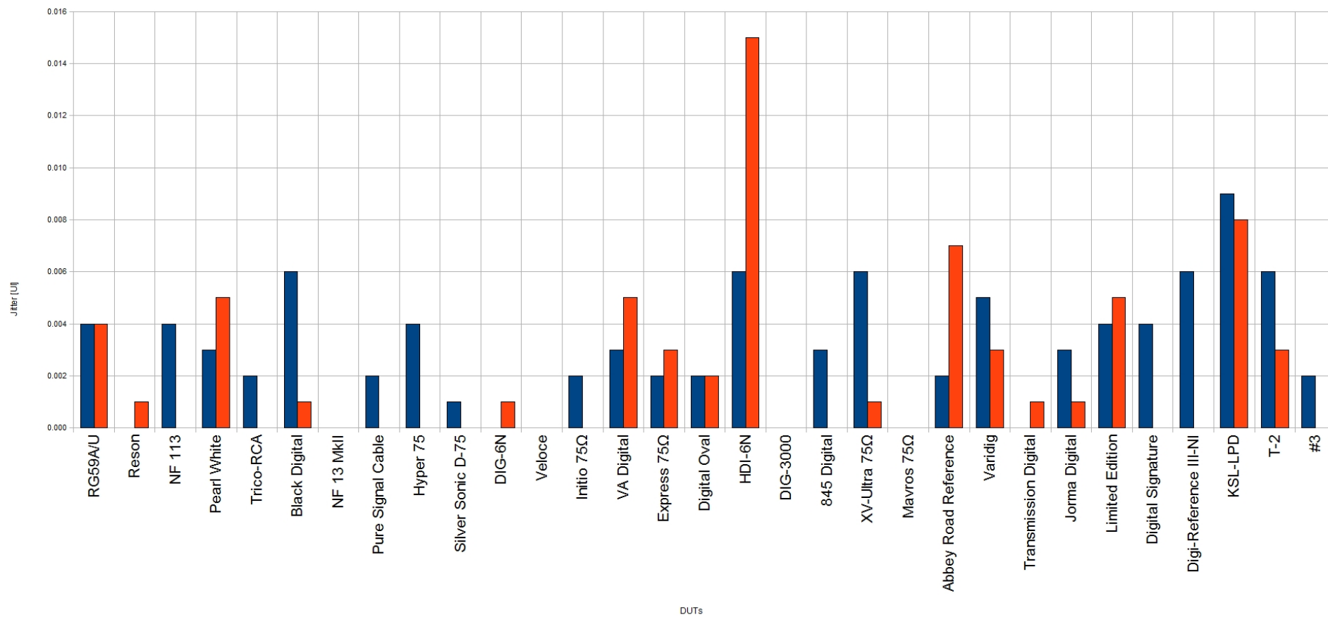
Καλώδια S/PDIF Coaxial Zero Crossing Jitter (44.1/88.2kHz)
