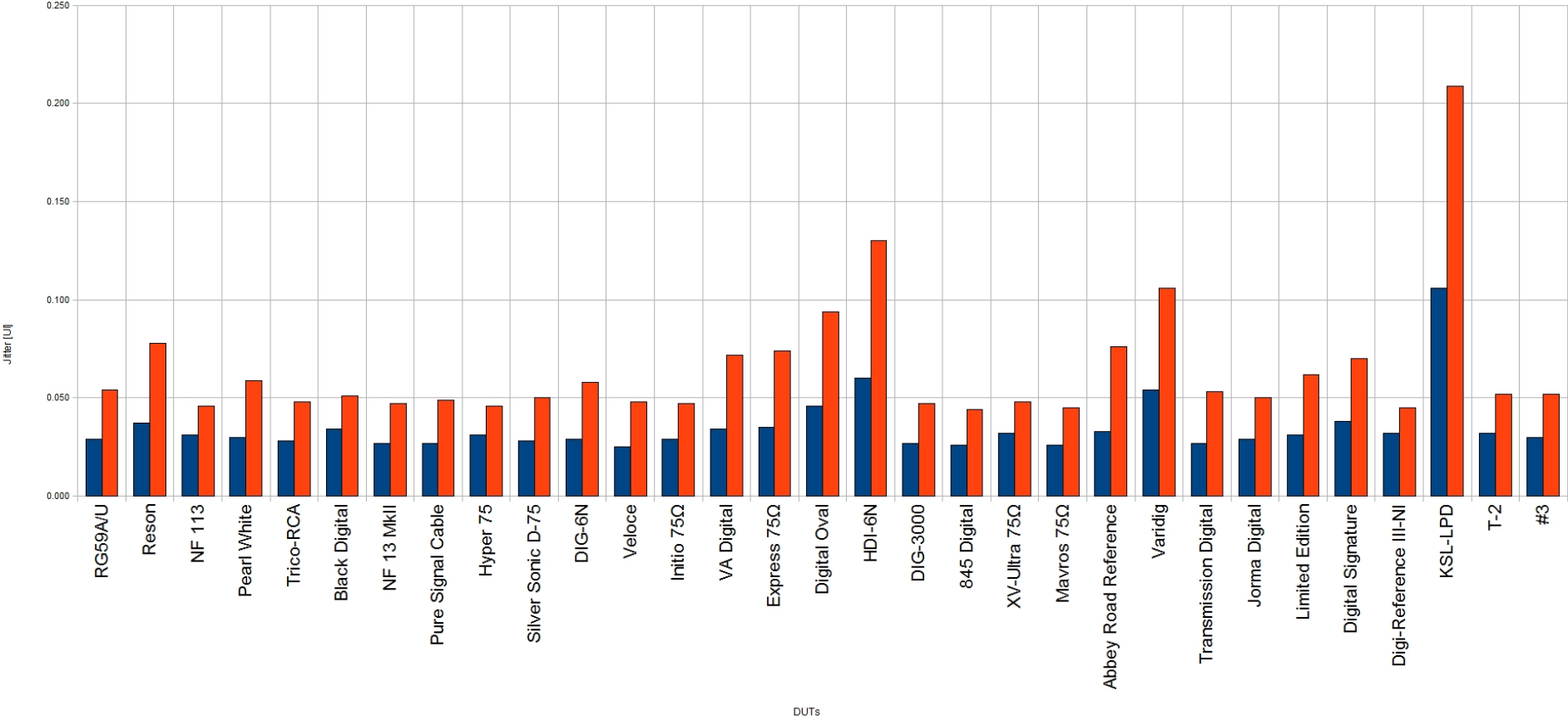
Καλώδια S/PDIF Coaxial Eye-Narrowing Jitter (44.1/88.2kHz)
